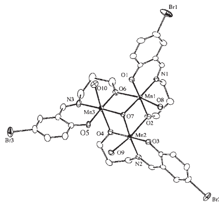
Figure 1. ORTEP drawing of 1 . Selected bond lengths ( \text{\AA} ) of the core structure: \text{Mn}(1)\text{-O}(2) 1.872(3), \text{Mn}(1)\text{-O}(1) 1.896(3), \text{Mn}(1)\text{-O}(7) 1.934(3), \text{Mn}(1)\text{-N}(1) 2.004(4), \text{Mn}(1)\text{-O}(6) 2.199(3), \text{Mn}(1)\text{-O}(8) 2.317(3), \text{Mn}(2)\text{-O}(4) 1.874(3), \text{Mn}(2)\text{-O}(3) 1.914(3), \text{Mn}(2)\text{-O}(7) 1.944(3), \text{Mn}(2)\text{-N}(2) 2.000(4), \text{Mn}(2)\text{-O}(2) 2.193(3), \text{Mn}(2)\text{-O}(9) 2.276(3), \text{Mn}(3)\text{-O}(6) 1.875(3), \text{Mn}(3)\text{-O}(5) 1.899(3), \text{Mn}(3)\text{-O}(7) 1.931(3), \text{Mn}(3)\text{-N}(3) , 2.008(4), \text{Mn}(3)\text{-O}(4) , 2.189(3), \text{Mn}(3)\text{-O}(10) 2.335(3).
